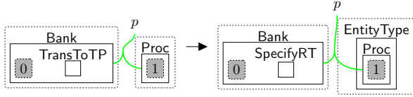
Fig. 29 senderType: specifying the type of Bank.
