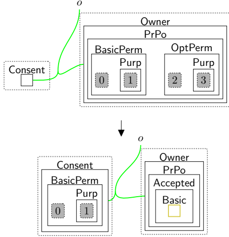
Fig. 6 acceptBasic : accepting only basic permissions and purposes.
