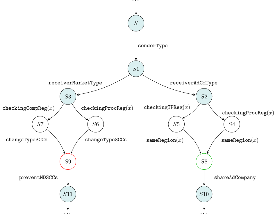
Fig. 28 Partial transition system illustrating the interaction between system and privacy rules. Teal states are produced by applying a system rule.
