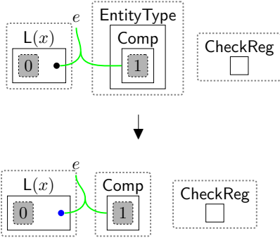
Fig. 54 \text{checkCompReg}(x) : checking the region of components, whether they are senders or receivers, by tagging their pointers, where x represents the name of a country or jurisdiction.
