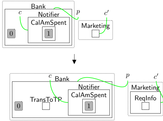
Fig. 48 branchReqInfo : Marketing requests the user's transaction details through ReqInfo . The entity TransToTP indicates that the system will transfer this data to Marketing.
