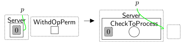
Fig. 51 checkConOptOut : after withdrawing the optional permissions, this rule generates the entity CheckToProcess to initiate the checking process of the permissions, allowing rule startCheck (Fig. 12) to be applied. This, in turn, changes the type of the third-party components to Comp_F ( changeTypeComp , Fig. 13). By doing so, any rule that shares data must match over Comp_F to ensure that the data is no longer shared following the user's request to stop sharing their data as shown in Fig. 39.
