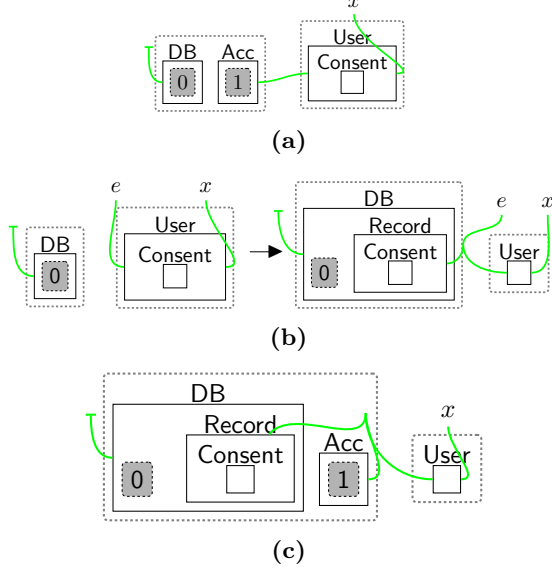
Fig. 2 (a) A bigraph modelling a database and account (with some abstracted contents) and a user wanting to register consent; (b) A rule allowing a user to pass consent to a database. The names allow any additional connections to the user; (c) the result of applying rule (b) to bigraph (a): the consent is moved from the user and added as a record in the database.
