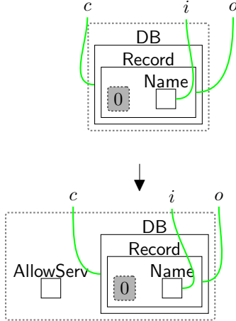
Fig. 44 provideServices : once the user registers with the system (their name is stored), then they are able to start using the system's services (AllowServ).
