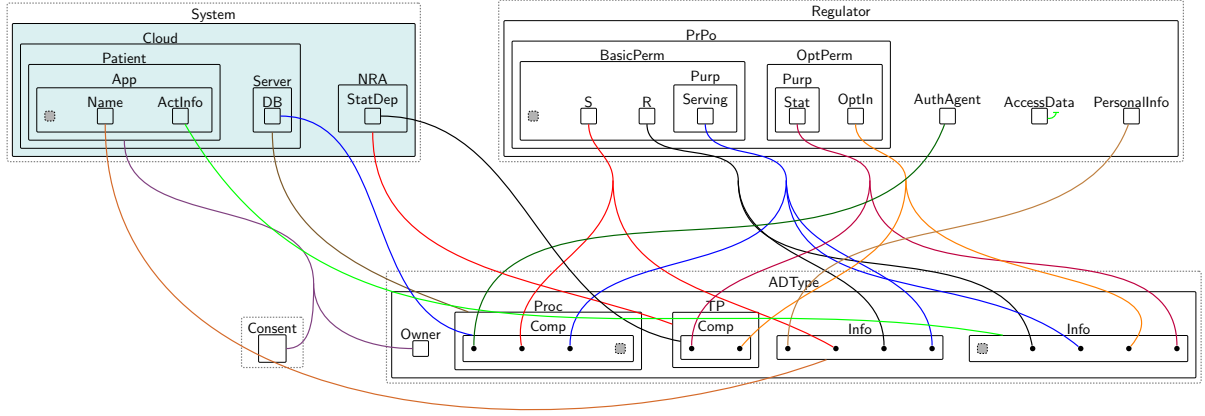
Fig. 37 A (partial) initial state of the cloud-based home healthcare system.
