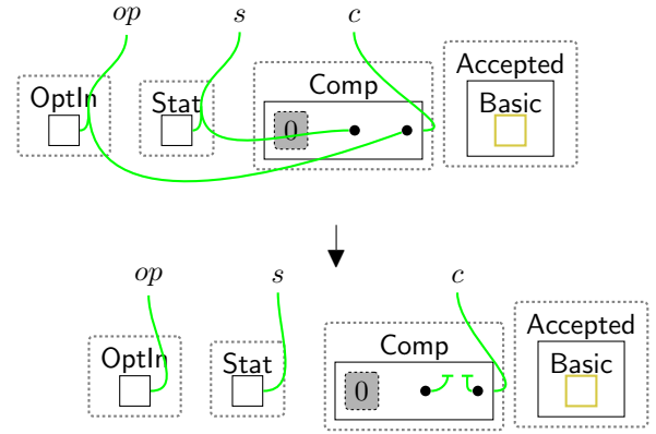
Fig. 50 closeLinks : this rule is applied when the user requests to opt out (stop sharing their data with the statistical department at the NRA). It closes the links to the optional permissions, indicating that the user withdraws them.
