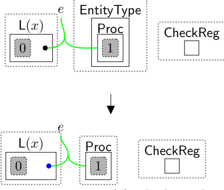
Fig. 15 checkingReg(x) : checking the region of the sender/receiver by tagging their pointers, where x is the name of a country or a jurisdiction.
