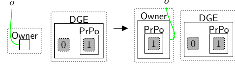
Fig. 4 sendPolicy : sending privacy policies to the data owner.
