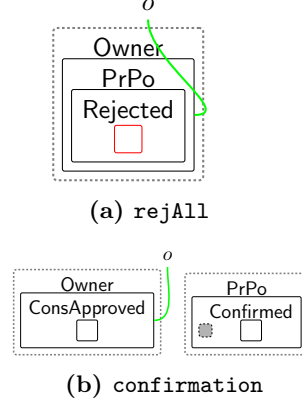
Fig. 41 Example bigraph patterns.
