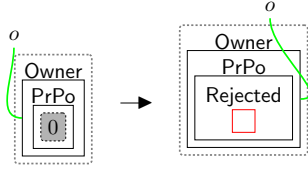
Fig. 10 rejectAll : rejecting all permissions and purposes.
