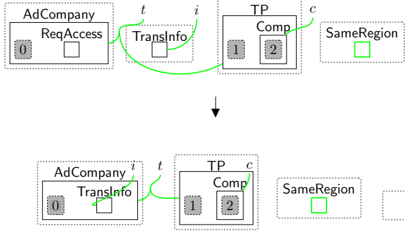
Fig. 33 shareAdCompany : sharing the data with AdCompany.
