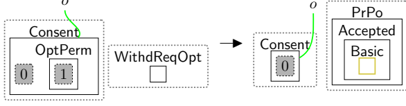
Fig. 22 processWithdOpt : the optional permissions are withdrawn and regenerate Basic to recheck the consent.
