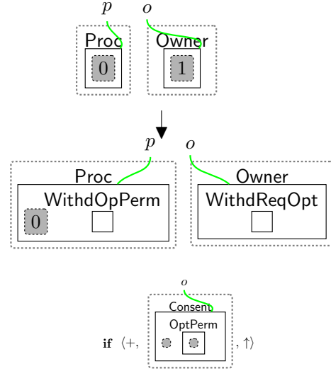
Fig. 21 withdrawReqOPT : the owner requests to withdraw the optional permissions. The condition allows the rule to be applied only if the owner has already accepted the optional permissions.
