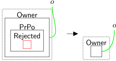
Fig. 43 changeDecisions : As the data owner could change their mind on policies in the future, this rule is used to reset the bigraph to a state where rule sendPolicy (Fig. 4) can be applied again.
