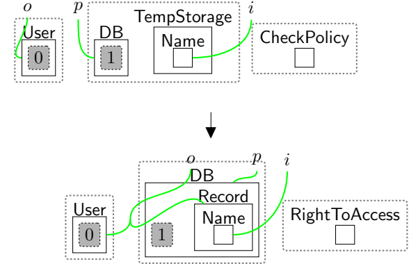
Fig. 24 storingName : storing the user's name.
