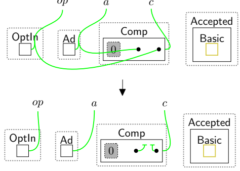
Fig. 7 closeLinks : remove links between rejected permissions.
