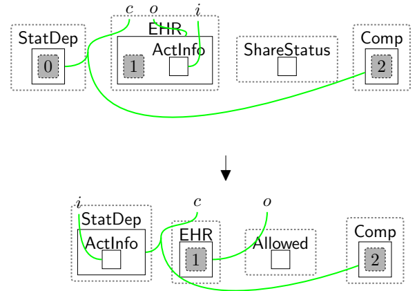
Fig. 38 shareActInfo : sharing the patient's activities information with the statistical department at the NRA.
