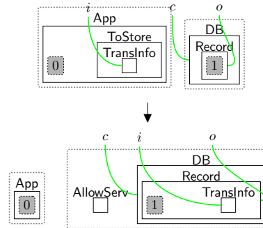
Fig. 47 storeTransInfo : the system stores the generated TransInfo in the user's Record. To allow the user to ask for a new service, AllowServ is created.
