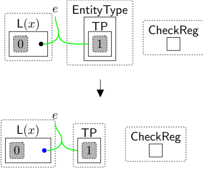
Fig. 53 \text{checkTPReg}(x) : checking the region of the third party, whether it is a sender or receiver, by tagging its pointer, where x represents the name of a country or jurisdiction.
