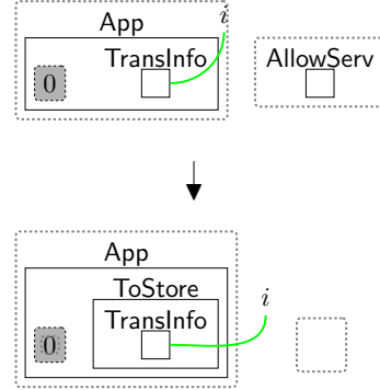
Fig. 46 generateTrans : when the transaction is generated, it should be stored in the DB. The entity ToStore is created to initialise the storing process in the DB.
