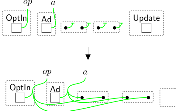
Fig. 11 confirm : confirming a DGE has evidence of data-owners consent.
