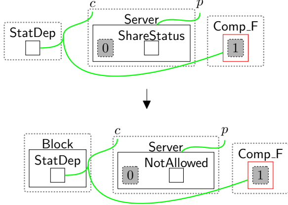
Fig. 39 preventshareActInfo : prevent sharing the patient’s activities information with the statistical department at the NRA.
