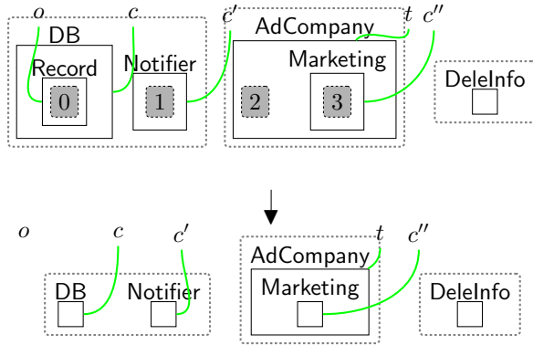
Fig. 35 deleteInfo : deleting the user's information after withdrawing the consent.
