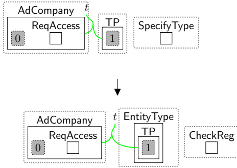
Fig. 31 receiverAdCmType: specifying the type of AdCompany.
