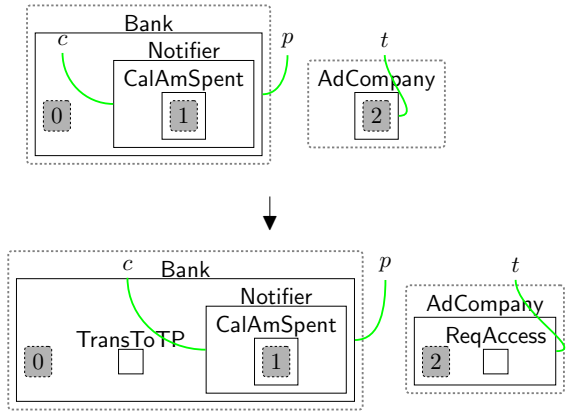
Fig. 49 adCompReqInfo : AdCompany requests the user's transaction details through ReqAccess . The entity TransToTP indicates that the system will transfer this data to AdCompany.
