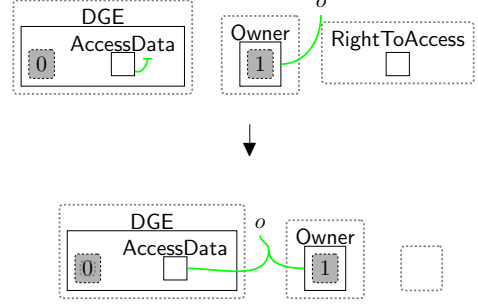
Fig. 14 rightToAccess : allowing the owner to ask the DGE for data access.
