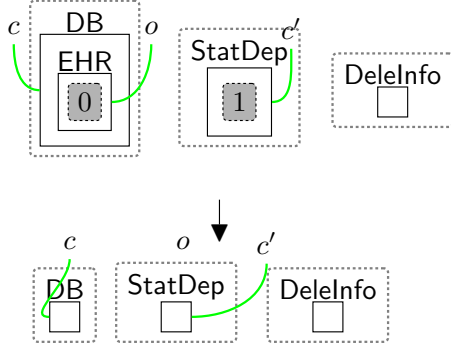
Fig. 40 deleteInfoEHR : deleting the patient’s information after withdrawing the consent.
