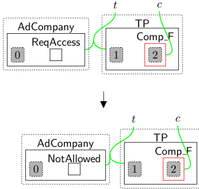
Fig. 26 preventAdCompany : prevent sharing the user's transaction information with AdCompany as the user rejects the optional permissions.
