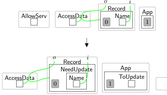
Fig. 25 updateReq : user's request to update their data.
