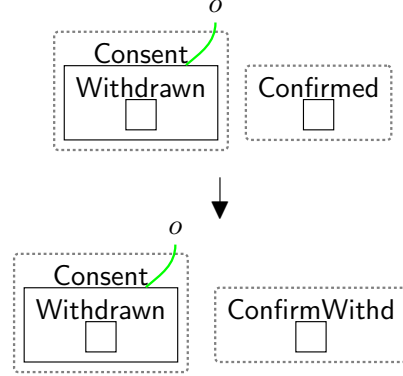
Fig. 20 confirmWithdrawal : acknowledgement of successful consent withdrawal.
