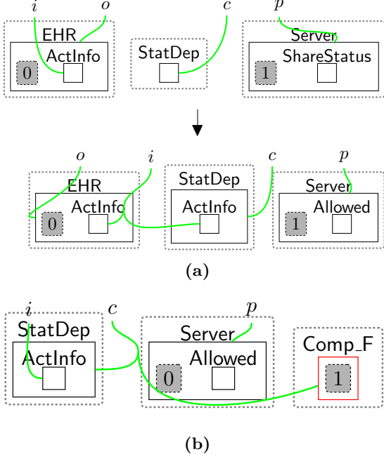
Fig. 42 (a) System-specific rule for copying data to a third-party. As the consent was not checked ( i.e. there is no match into the privacy perspectives), this may result in a privacy violation; (b) Partial model state showing the privacy violation: transaction information has moved when consent was not given.
