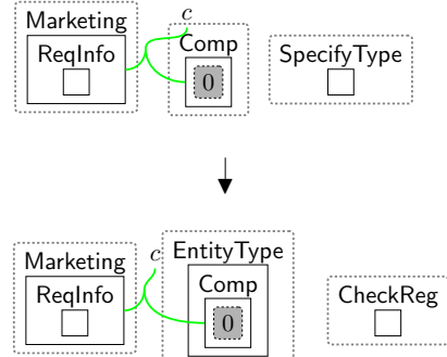
Fig. 32 receiverMarketType: specifying the type of Marketing.
