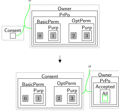
Fig. 5 acceptAll : accepting all permissions and purposes.
