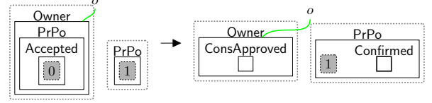
Fig. 11 confirm : confirming a DGE has evidence of data-owners consent.
