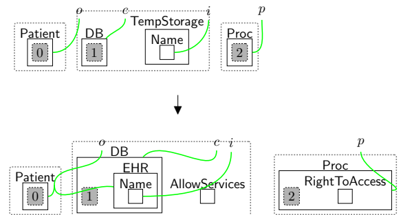
Fig. 52 storingName : as the CCPA considers the patient to have consented to share their data, the patient's name is stored directly once the user registers with the system. Unlike rule storingName Fig. 24, where the entity CheckPolicy is replaced with RightToAccess , this rule does not include CheckPolicy since no consent is required to check. Therefore, it generates the entity RightToAccess to allow rule rightToAccess (Fig. 14) to be applied.
