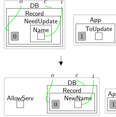
Fig. 45 updatingName : the system updates the user's name by replacing Name with NewName. Note that the new name should have the same permissions of the previous name as it is derived information. The entity AllowServ is generated again to allow the user to ask for a new service.
