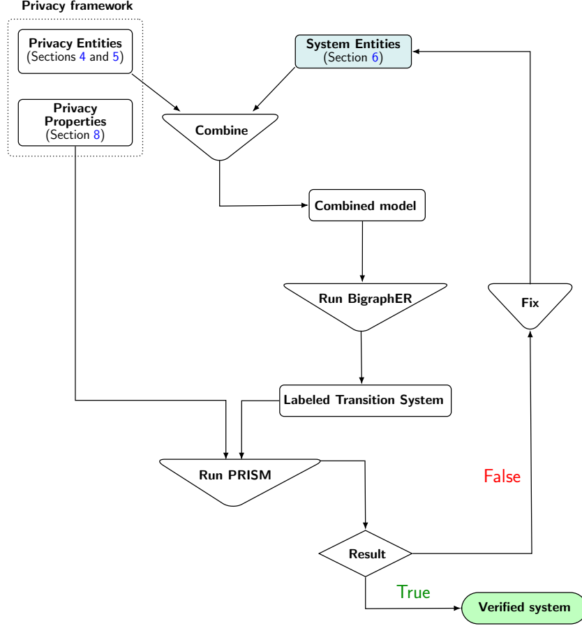
Fig. 1 Bigraph-based privacy framework: The teal box represents the user-specified elements. These elements are combined with the privacy rules and entities to form a unified model. BigraphER then analyses this unified model to generate a labelled transition system. The model is subsequently verified using the PRISM model checker to assess its compliance with the specified privacy properties. If the verification result is positive, the system is considered to meet the privacy properties. If the result is negative, the system must be revised to address the identified issues, after which it undergoes reanalysis. This iterative process continues until the system successfully passes verification.
