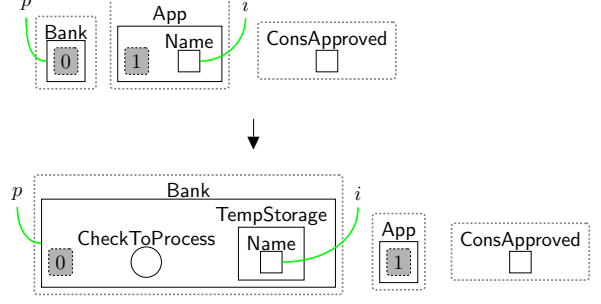
Fig. 23 registerRequest : user's registration with the system.
