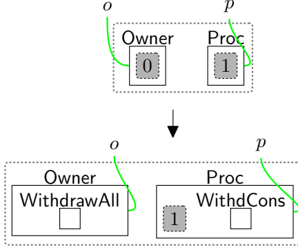
Fig. 18 withdrawReq : the owner requests to withdraw all permissions.
